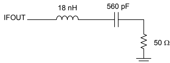
Figure 17. IFOUT 50 \Omega Matching Network
